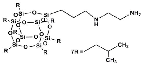
Aminoethylaminopropylsilyl POSS (POSS3)
